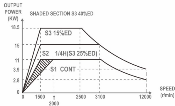
OUTPUT POWER-SPEED CHARACTERISTIC NORMAL
