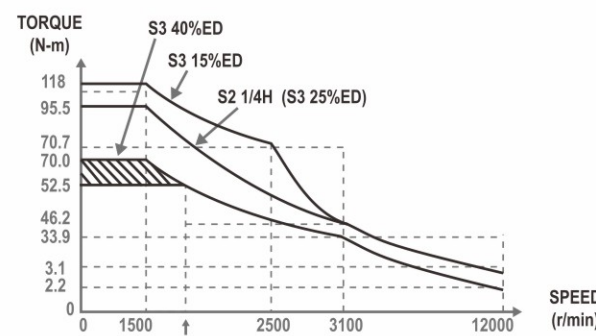
TORQUE-SPEED CHARACTERISTIC NORMAL
