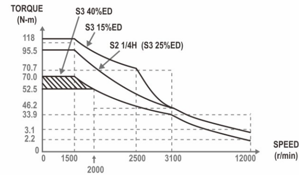
TORQUE-SPEED CHARACTERISTIC NORMAL
